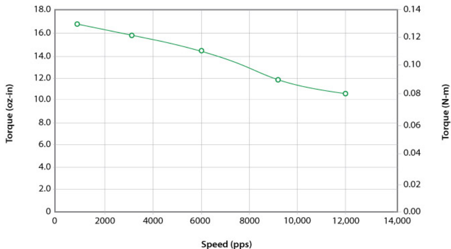
211-20-02 24VDC, 1.3 Amps/Phase, Bipolar, 1/2 Stepping
